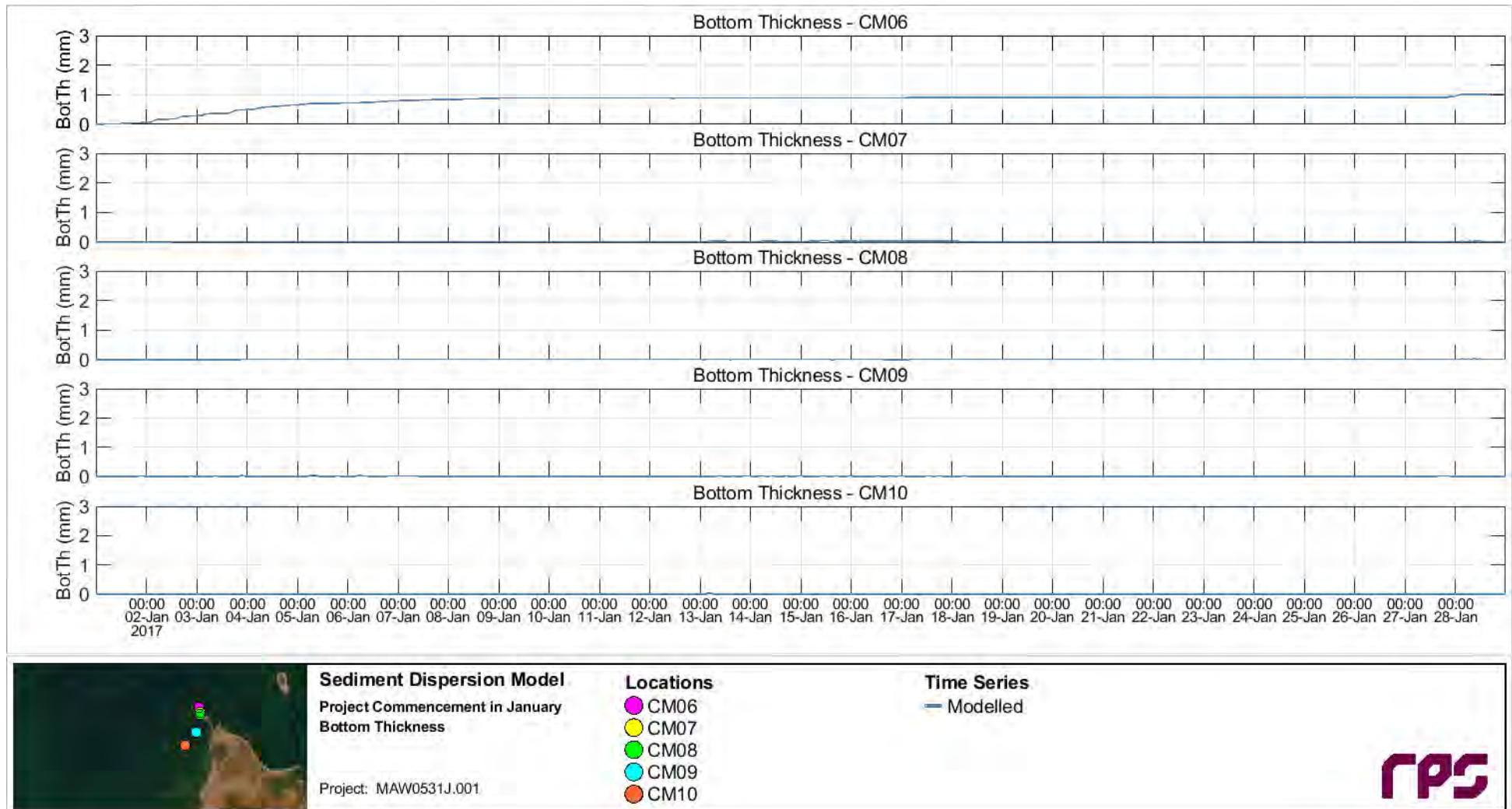
Figure 5.97 Time series of predicted dredge-excess bottom thickness at the CM06 to CM10 sites throughout the entire Scenario 4 duration (1 to 29 January 2017).
