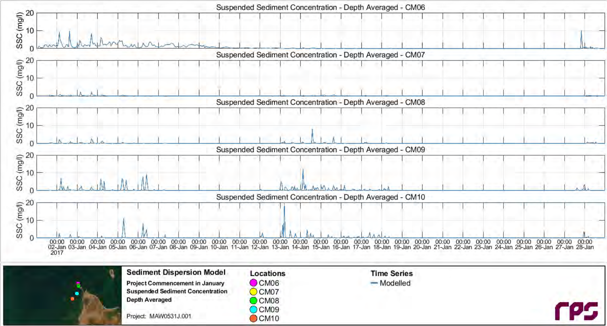
Figure 5.72 Time series of predicted dredge-excess depth-averaged TSSC at the CM06 to CM10 sites throughout the entire Scenario 4 duration (1 to 29 January 2017).
