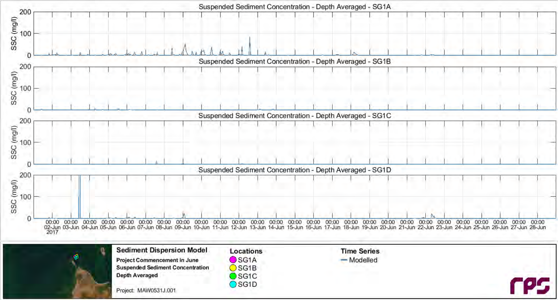
Figure 5.59 Time series of predicted dredge-excess depth-averaged TSSC at the SG1A to SG1D sites throughout the entire Scenario 1 duration (1 to 29 June 2017).
